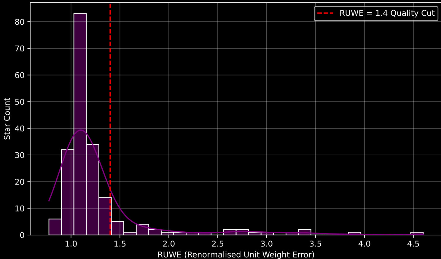
GAPOGEE DR17 Field [008+53_MGA] RUWE Distribution (n= 196)
