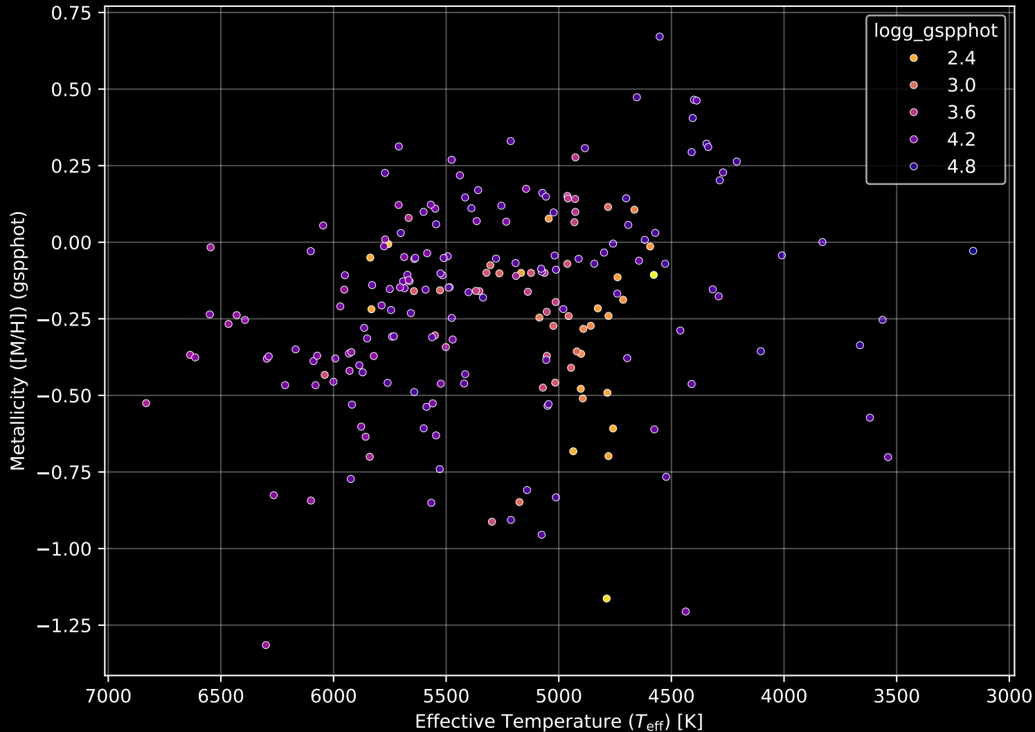
APOGEE DR17 Field: [008+53_MGA] Stellar Population Parameters (n= 211)
