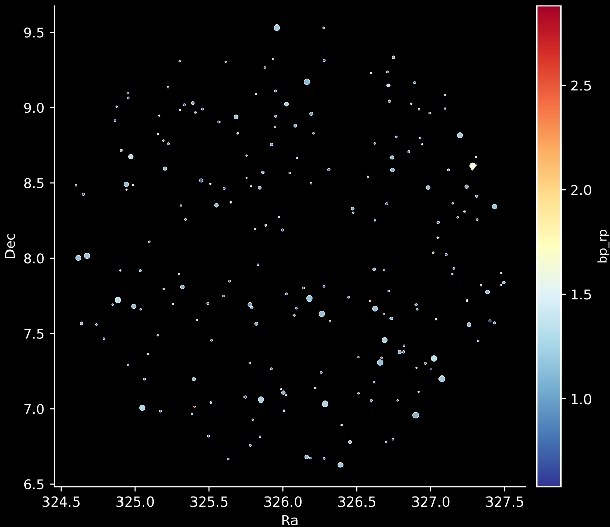
APOGEE DR17 Field: [008+53_MGA] Stars: 211
