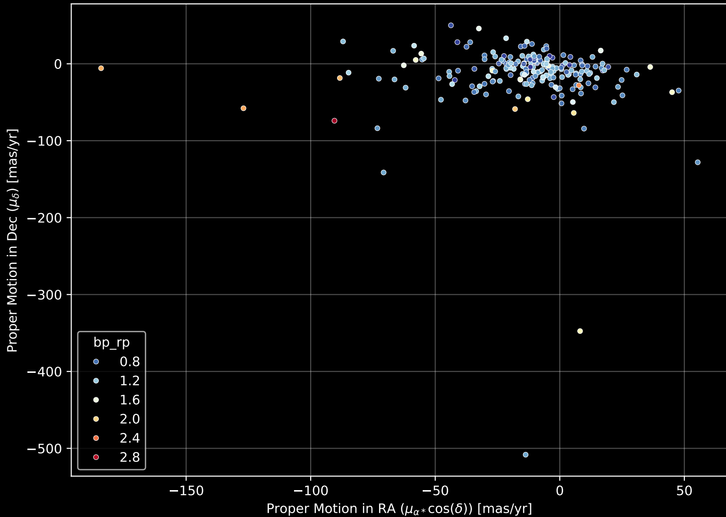
APOGEE DR17 Field: [008+53_MGA] Proper Motion Diagram (n= 211)
