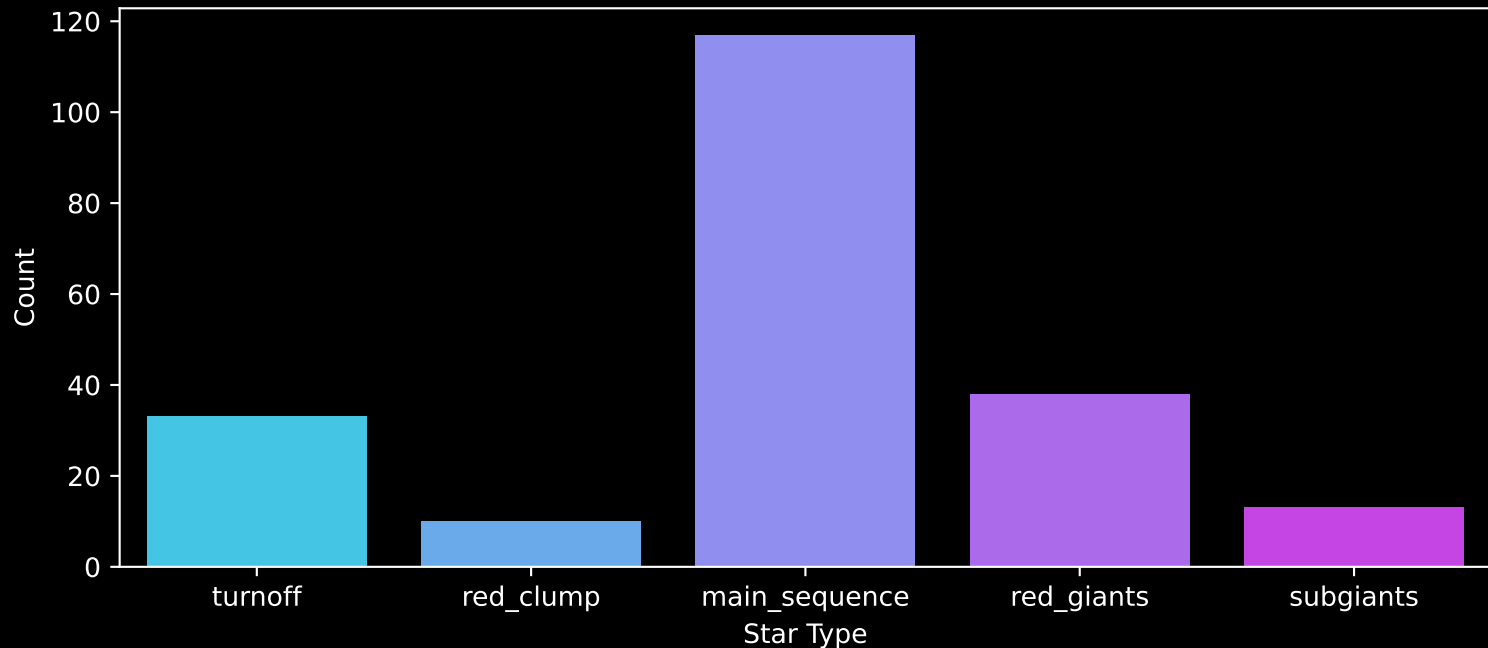
APOGEE DR17 Field: [008+53_MGA] Count plot of Star Type
