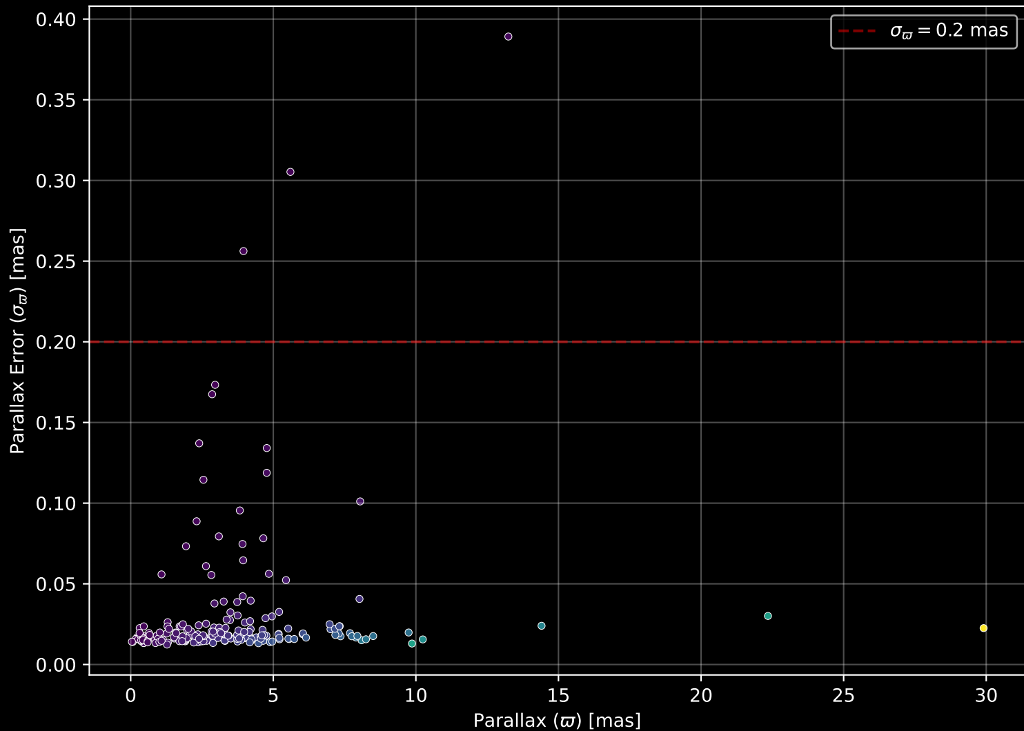
APOGEE DR17 Field: [008+53_MGA] Parallax Quality (n= 211)
