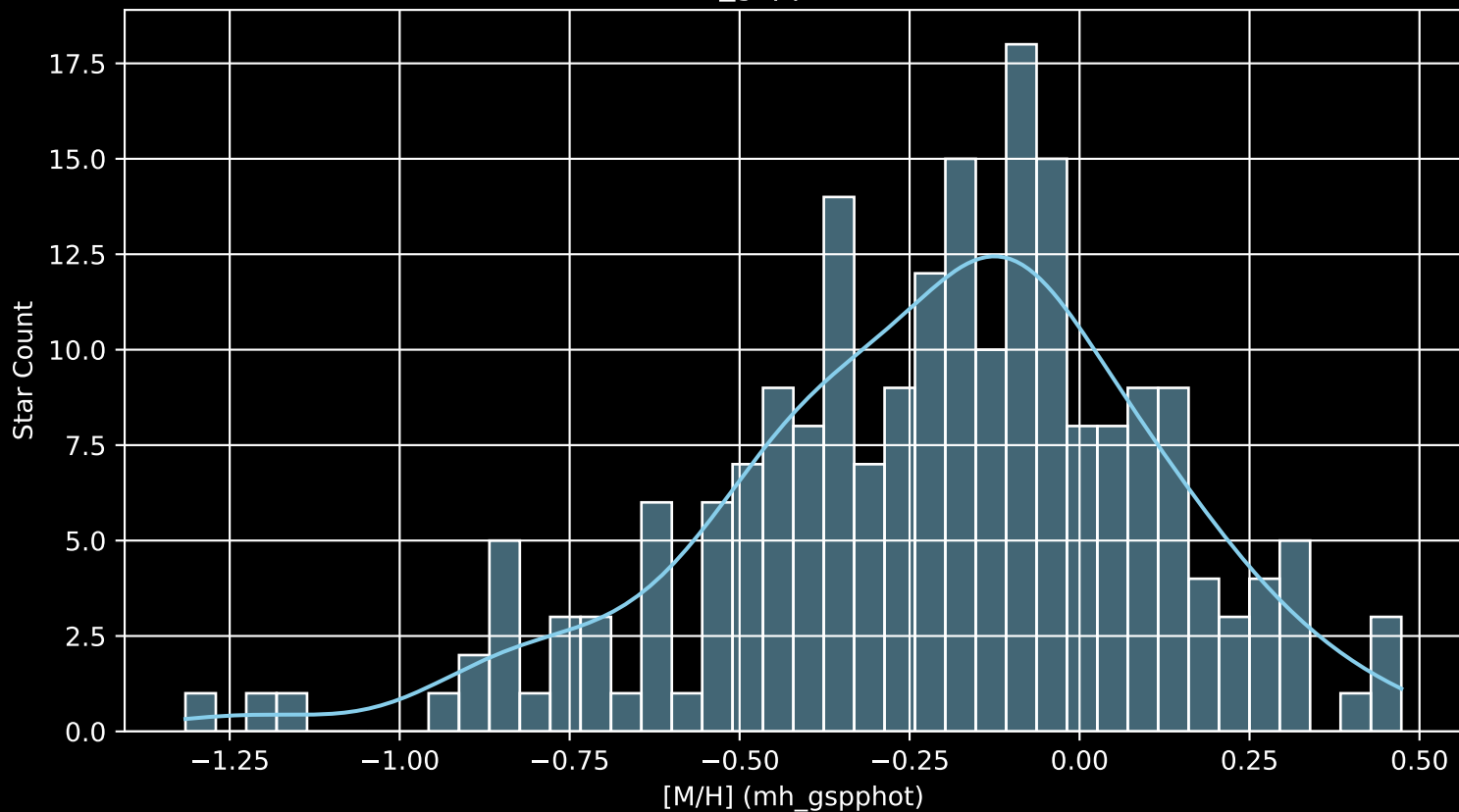
APOGEE DR17 Field: [008+53_MGA [M/H] (mh_gspphot) (n= 210)
